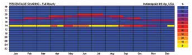
Figure 4: Horizontal Louvers
