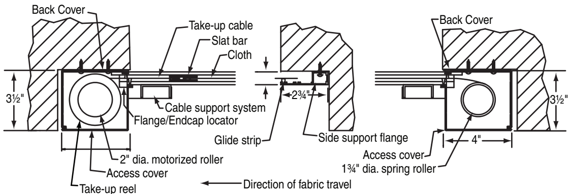
Typical Outside Installation-Boxes Down
