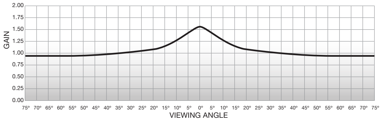
GAIN CHART TECVISION XT1600X WHITE NANOPERF
