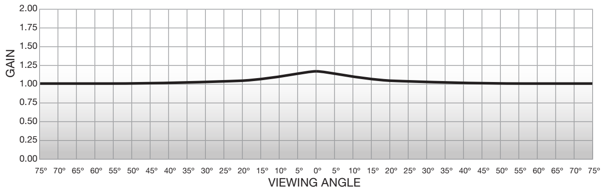
GAIN CHART TECVISION XT1100X WHITE
