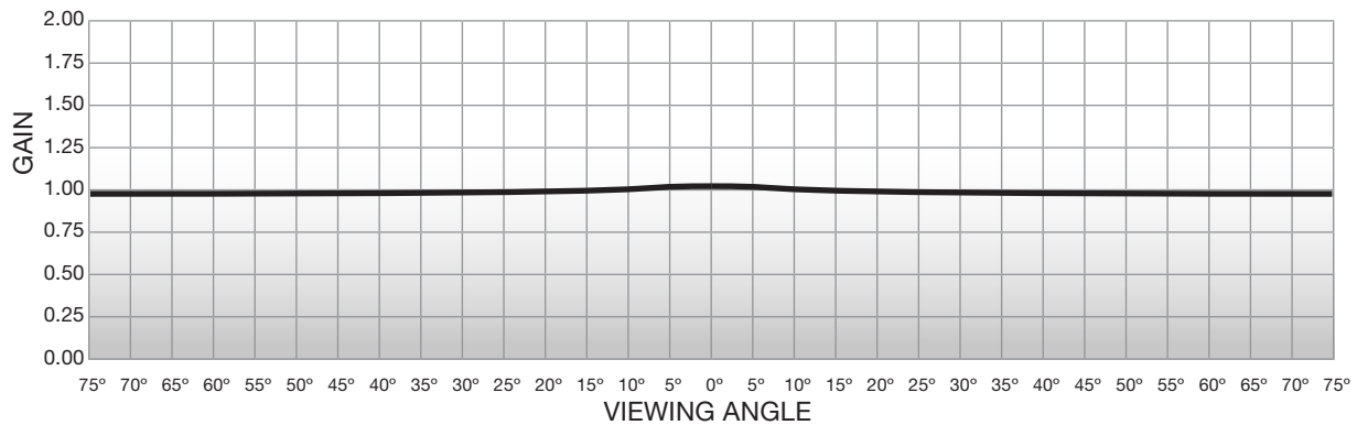
GAIN CHART TECVISION XT1000X WHITE
