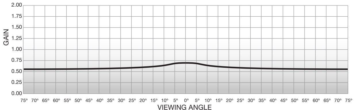
GAIN CHART TECVISION XH700X GREY
