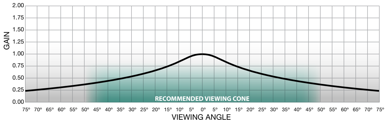
GAIN CHART TECVISION MS1000X ALR
