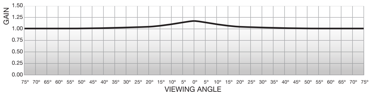
GAIN CHART TECVISION XT1100X WHITE
