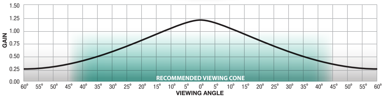
GAIN CHART: 0° GAIN: 1.2, VIEWING CONE: 60° CINEFLEX CH1200 V
