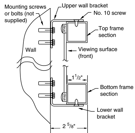
Cross section of mounted unit
