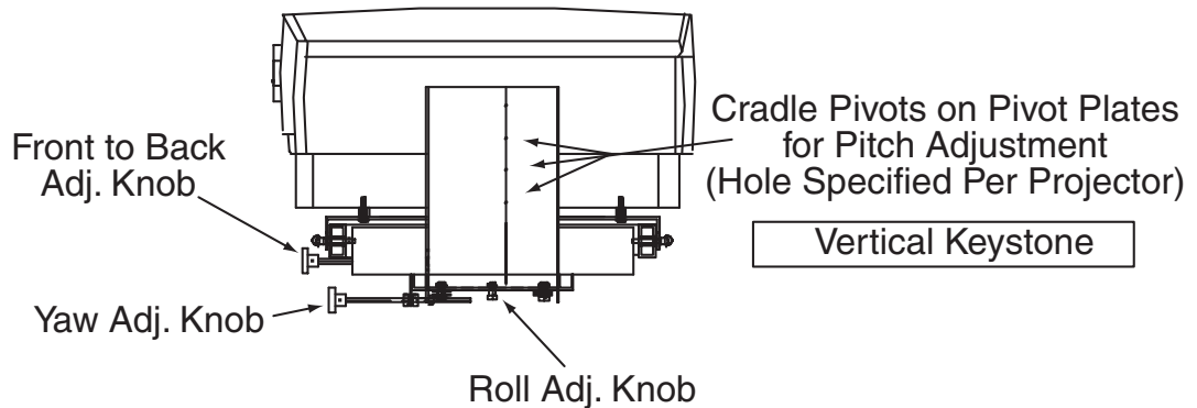
Side Elevation
