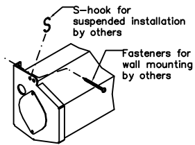
Isometric Mounting Detail
