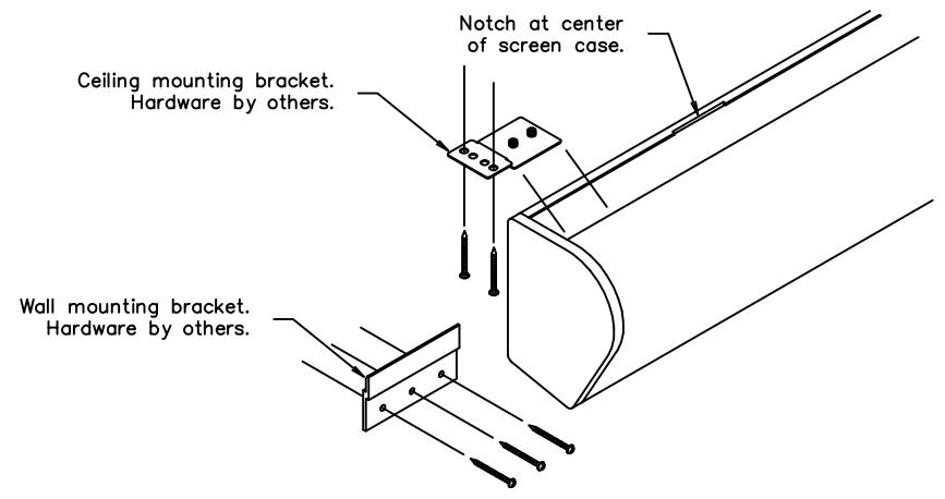
Mounting Detail Not To Scale
