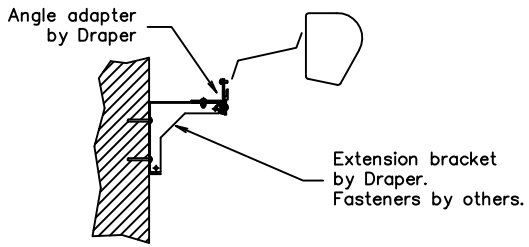
Mounting Details
