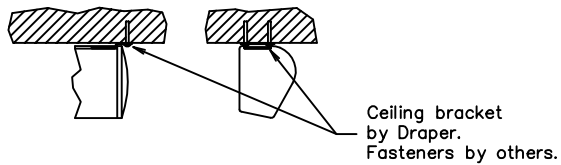
Ceiling Mounting
