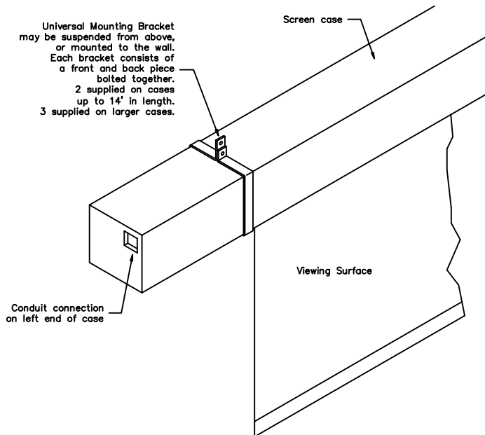
Mounting Details
