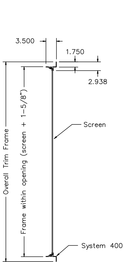
Section
