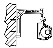
Wall Mounting with Extended Bracket
