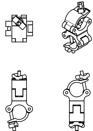
2" DOUBLE CHEESEBOROUGH CLAMP
