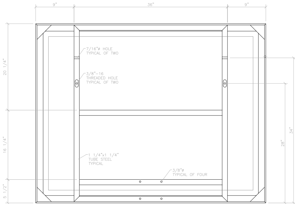
REAR VIEW
