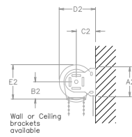
DRAPER MANUAL FLEXSHADE Dimensions & Data
