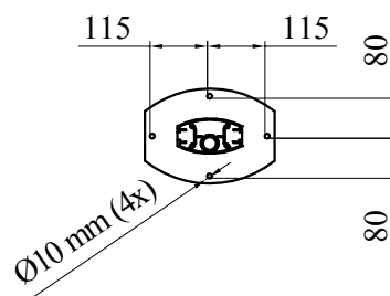
Ceiling hole pattern
