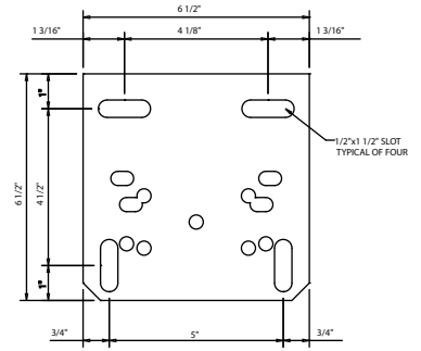
BOLT PATTERN DETAIL
