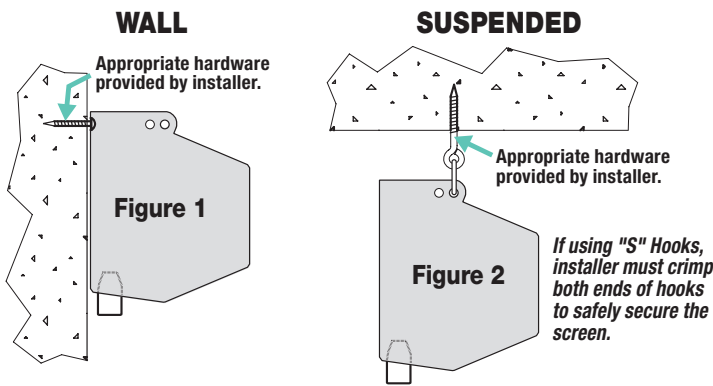
Wall Installation (Fig. 1)
