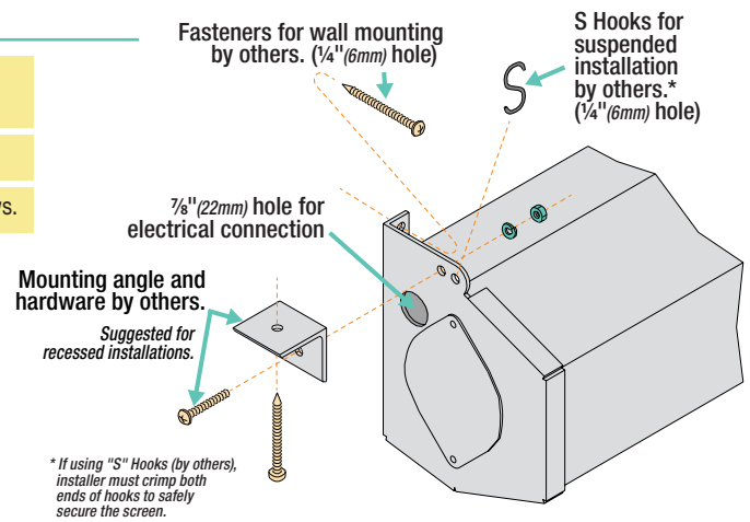
Wall Installation (Fig. 1)
