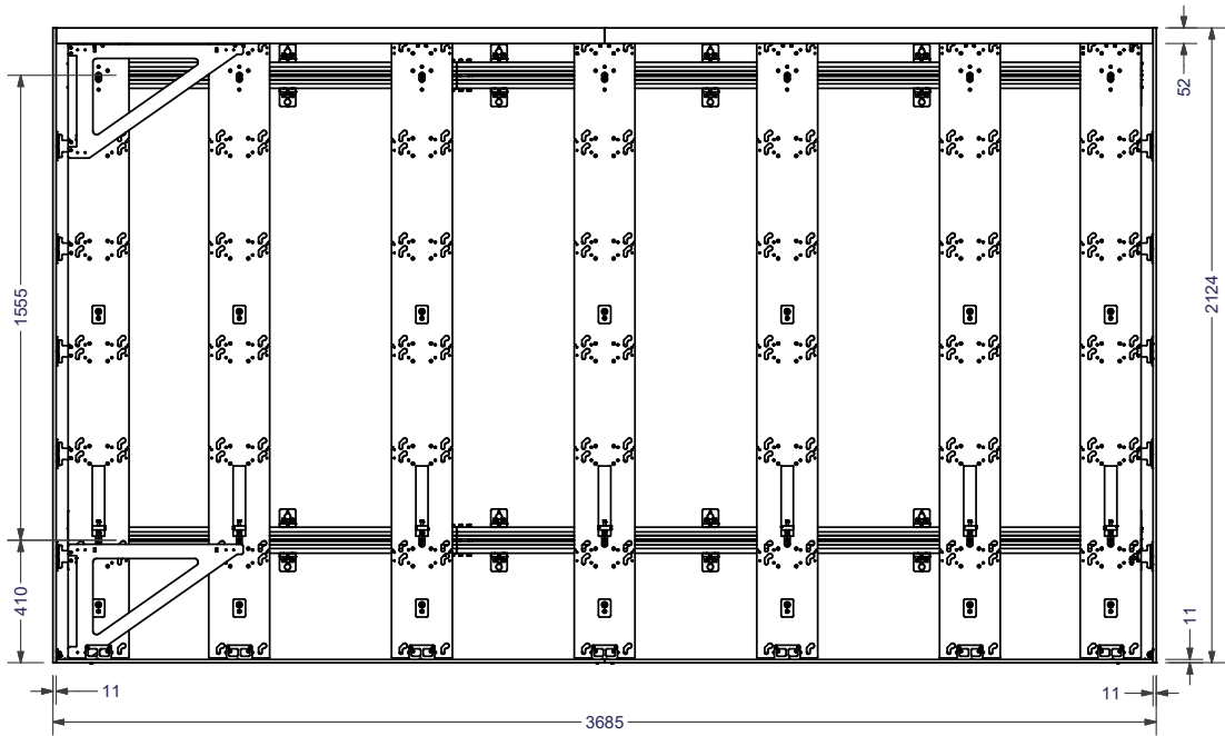
FRAME WITH TRIM
