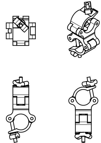
2" DOUBLE CHEESEBOROUGH CLAMP (QTY 1 - 232180) (QTY 4 - 232181)
