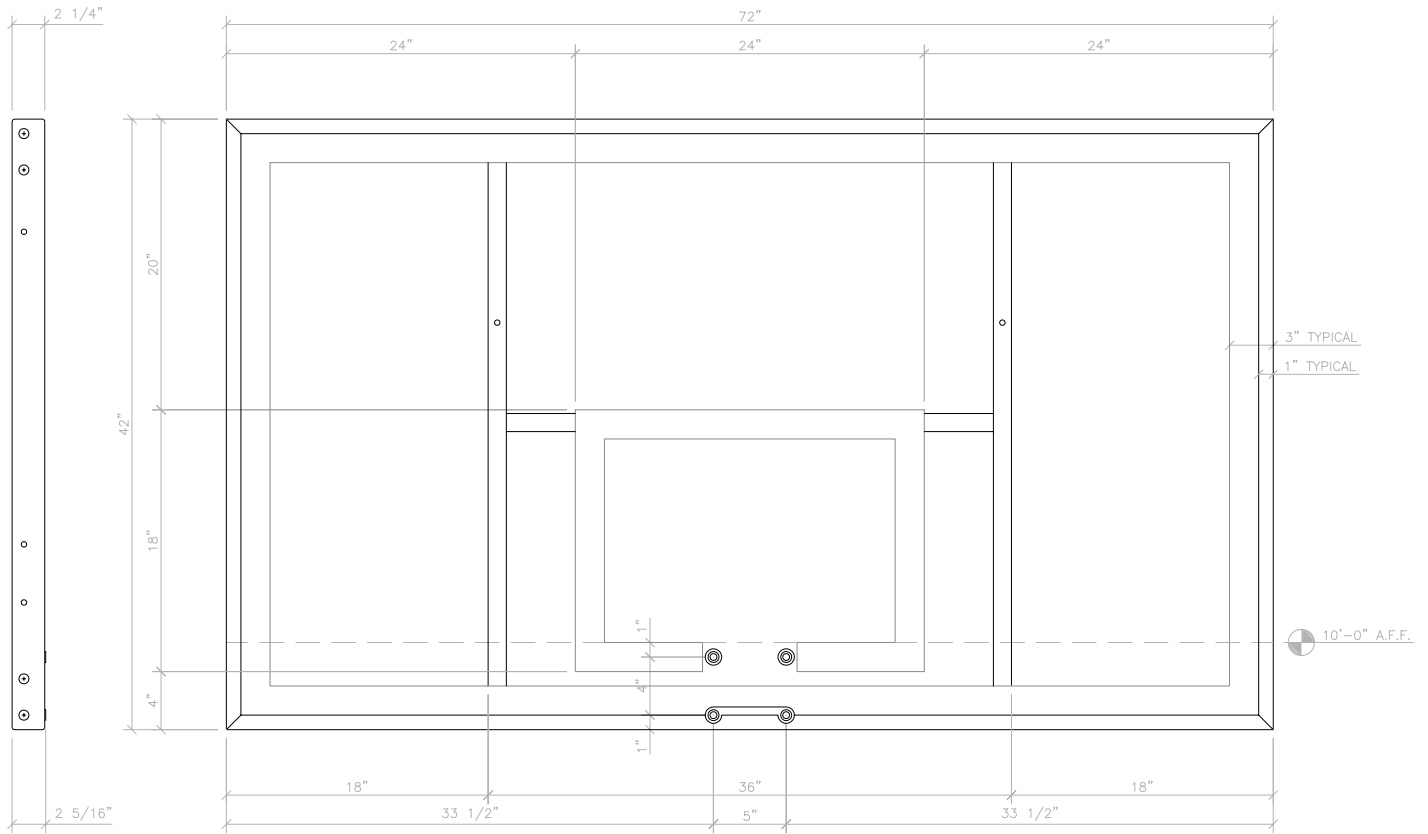
SIDE VIEW
