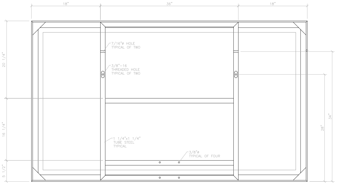
REAR VIEW
