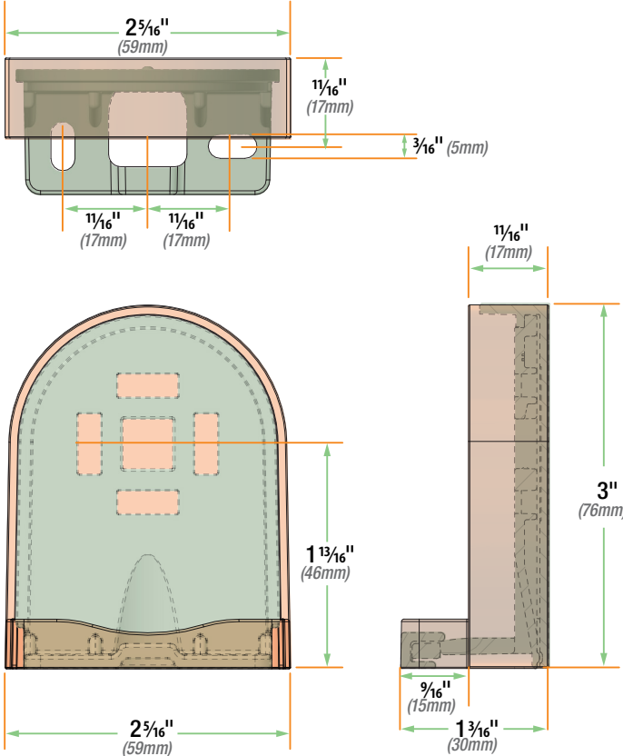
C002.1820 (Motor End, Extended)
